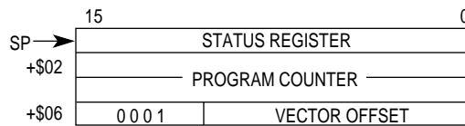
Figure B-4. Throwaway Four-Word Stack Frame, Format $1
